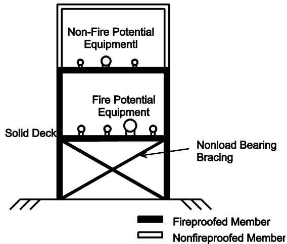
Figure 1. Structure Supporting Equipment In Fire Exposed Area.
