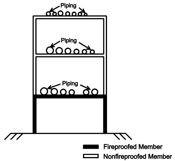
Figure 2. Pipe Rack With No Pumps Beneath.
