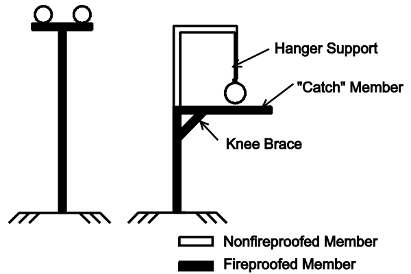
Figure 6. Small Pipe Racks.
