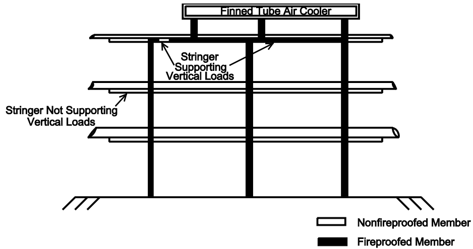
Figure 4. Pipe Rack Supporting Finned Tube Air Cooler (Side View).
