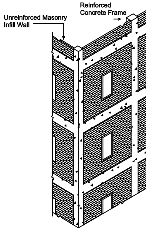
Figure 5. Concrete Frame With URM Infill. (Federal Emergency Management Agency Publication FEMA 154, March 2002, Rapid Visual Screening of Buildings for Potential Seismic Hazards.)
