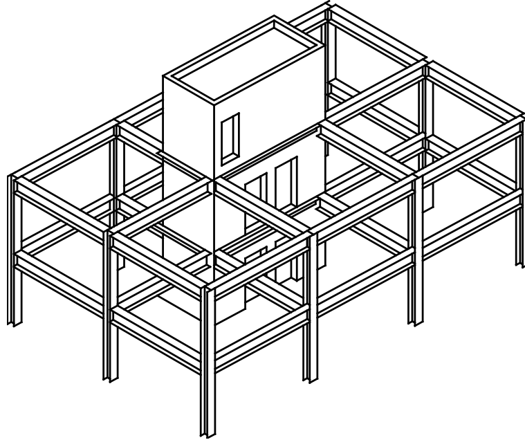
Figure 3. Steel Frame With Shear Wall. (Federal Emergency Management Agency Publication FEMA 154, March 2002, Rapid Visual Screening of Buildings for Potential Seismic Hazards.)
