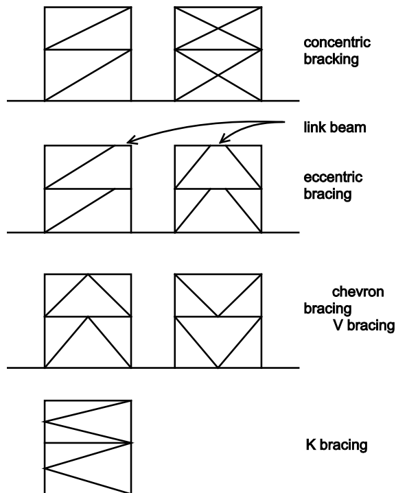
Figure 4. Bracing Types. Federal Emergency Management Agency Publication FEMA 547, October 2006; Techniques for Seismically Rehabilitating Existing Buildings.
