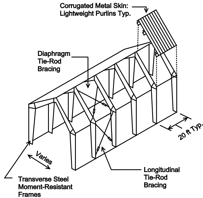
Figure 6. Light Metal Construction. (Federal Emergency Management Agency Publication FEMA 154, March 2002, Rapid Visual Screening of Buildings for Potential Seismic Hazards.)
